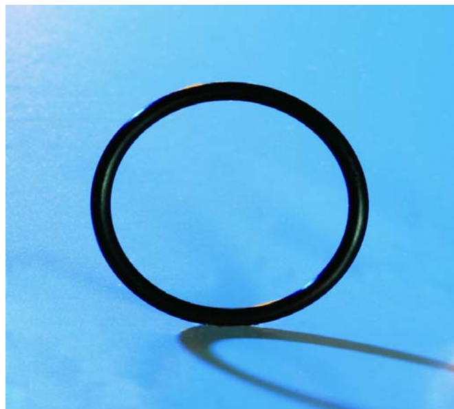
Black Specialty Fluoroelastomer Service Temperature Range: -30°C to 220°C
